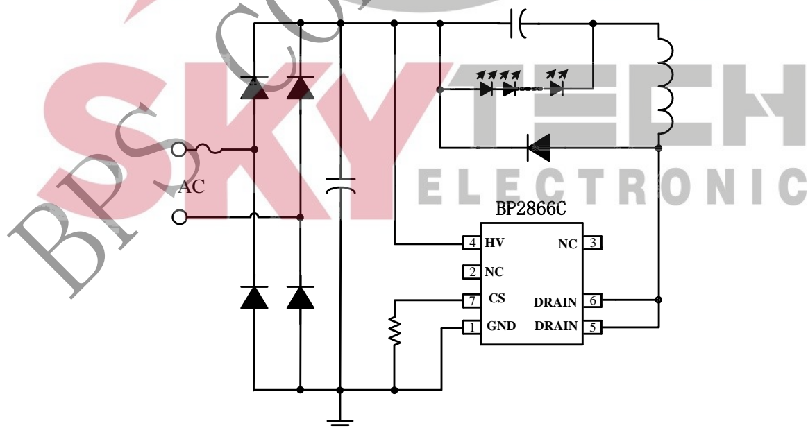
Figure 1. Typical application circuit for BP2866C
